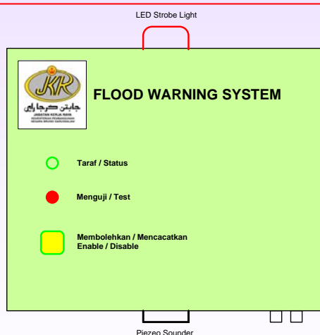
Indicator Panel
